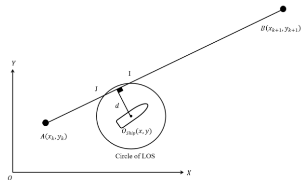
Figure 2: Illustration of the LOS circle and way path
