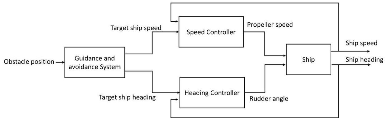
Figure 6: Guidance, avoidance and control block diagram for the ship
