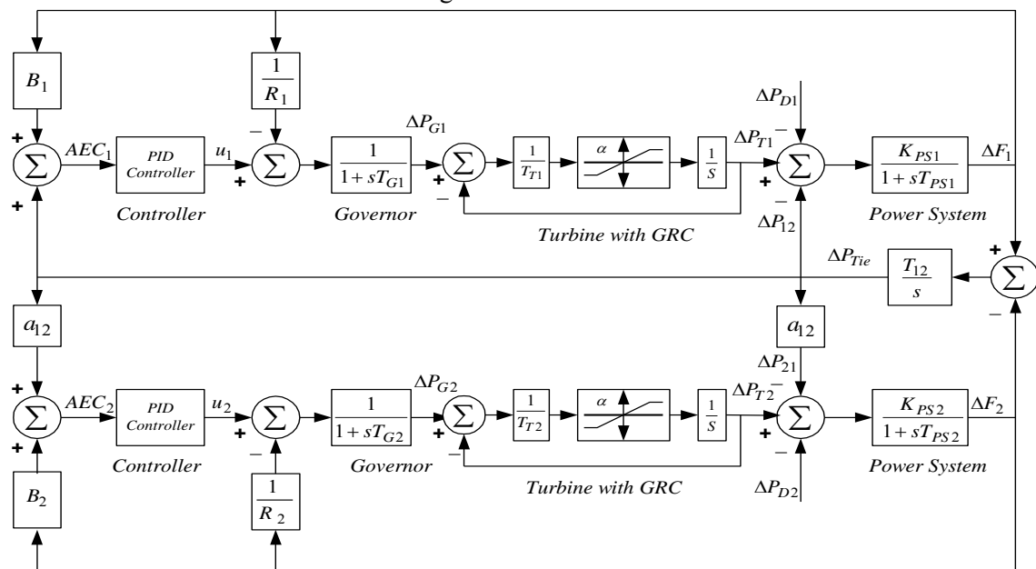
Figure-1 Two area thermal power plant
