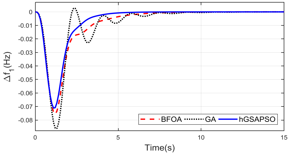
Fig.6 Variation of frequency for area-1 under case-2
