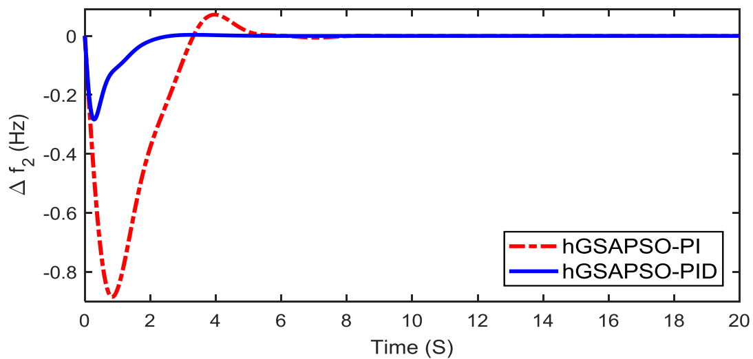
Figure-17: Frequency variation response of area-2 without GRC
