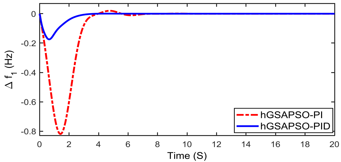
Figure-16: Frequency variation of area-1 without GRC
