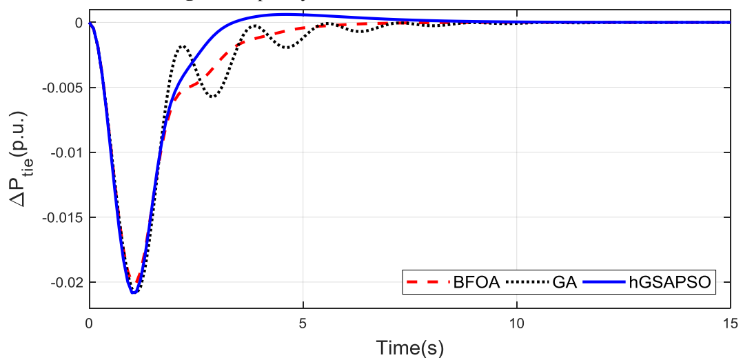
Fig.11 Tie line power deviation under Case-3
