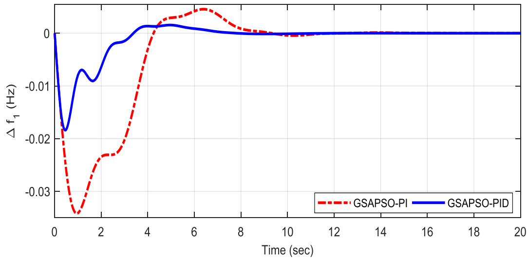
Figure-19: Frequency variation response of area-1 with GRC
