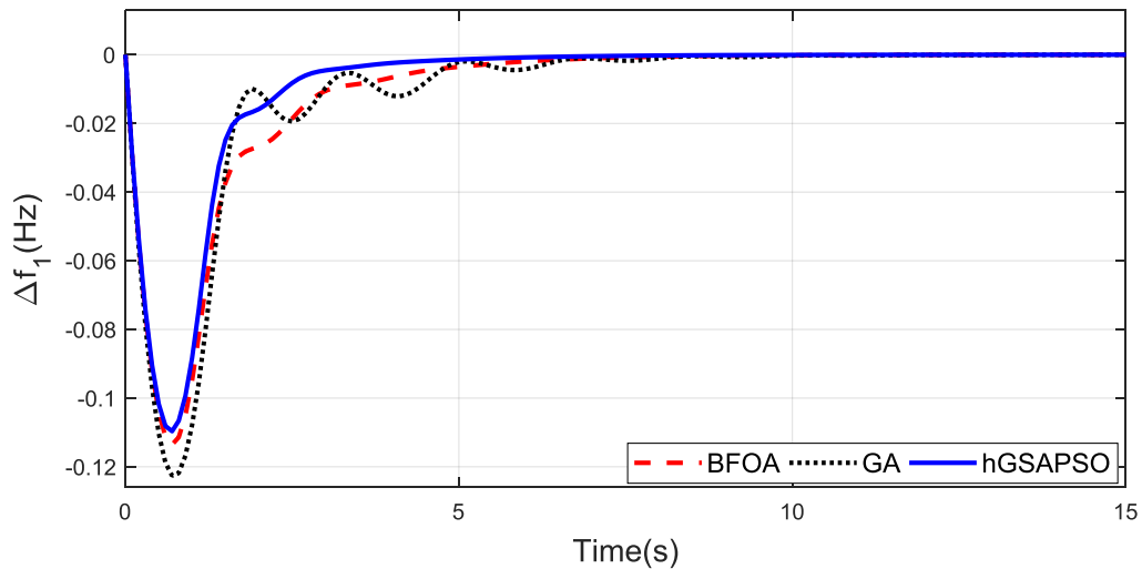
Fig.9 Frequency deviation in area-1 under case-3
