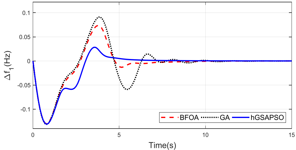
Figure-12: Frequency response in area-1 under Case-4
