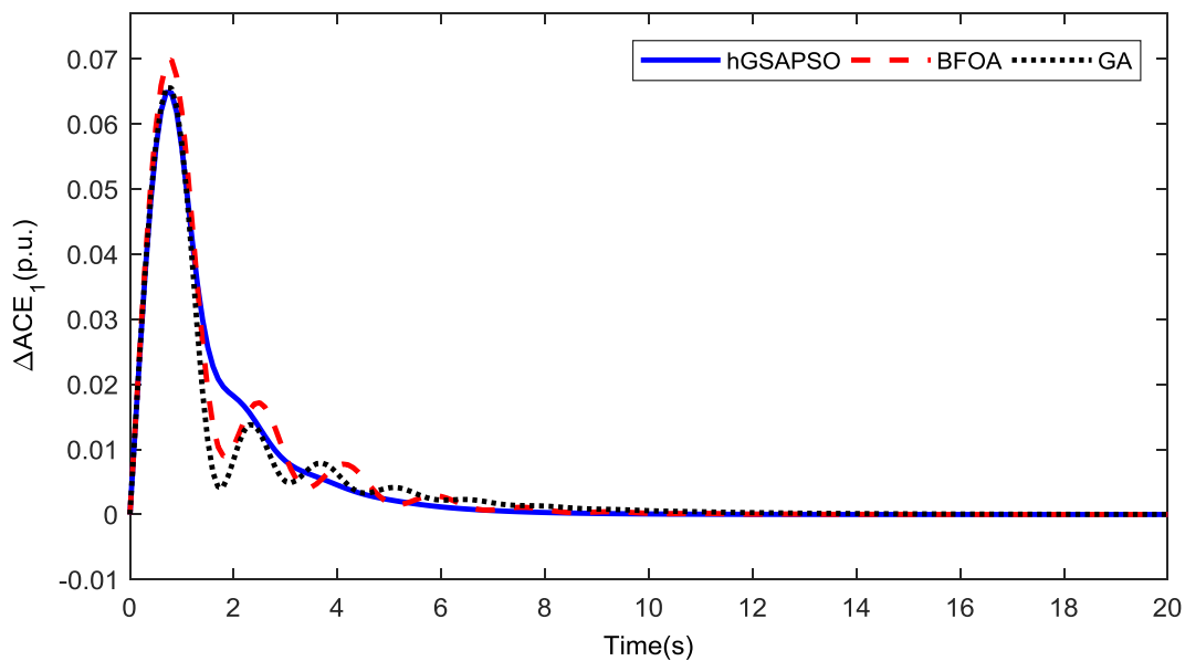
Fig.5. ACE-1 under case-1
