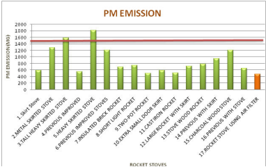
Fig. 24. Particulate Matter Emissions to Complete WBT (milligrams).
