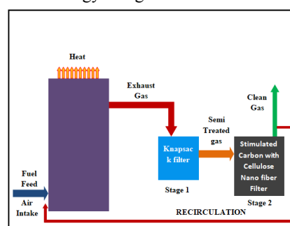
Fig. 4. Proposed Methodology
