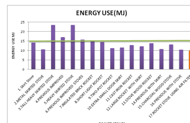
Fig. 21. Energy Use for Stoves to Complete the WBT (Mega Joules). Suggested Fuel (Energy) Use Benchmark: The improved cook stove should use less than 15 MJ of energy to complete the 5-IWBT.
