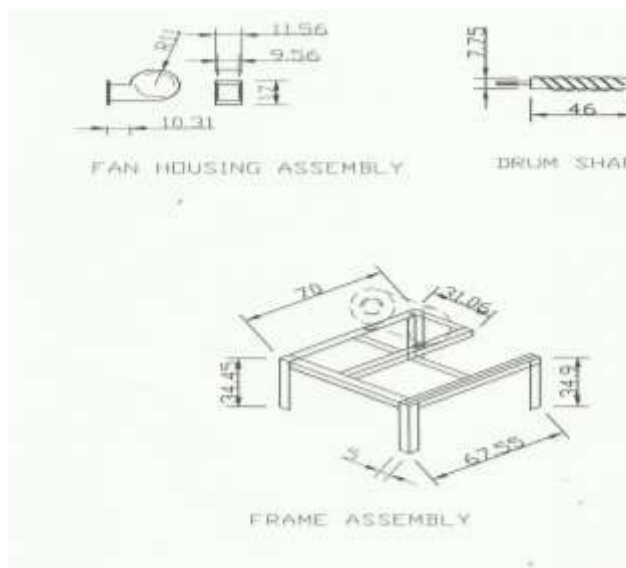
Fig.2: Components assembly
