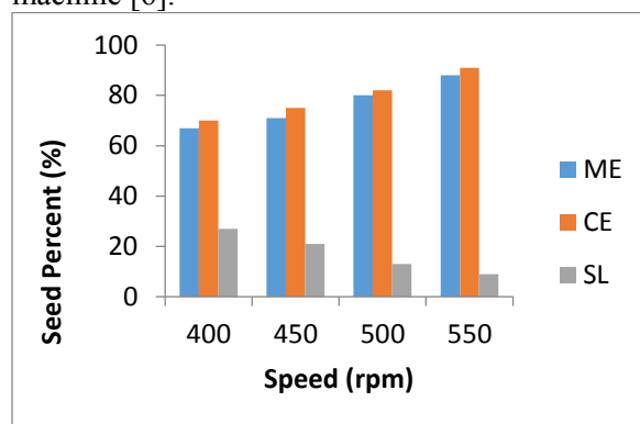
Fig. 5: Effect of speed on machine performance
