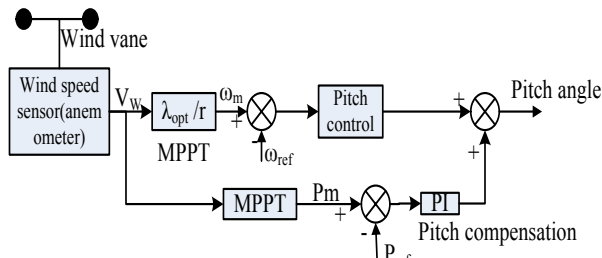
Fig.2.4. Block diagram of pitch angle control Adama-I wind turbine
