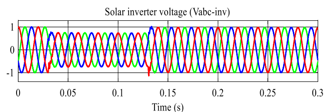
(a) Grid connected PV-STATCOM three phase output voltage (p.u) during daytime
