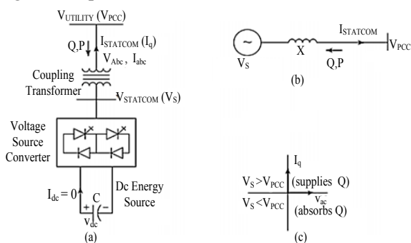
Fig.1.4. the STATCOM principle of operation diagram: (a) a power circuit, (b) an equivalent circuit, (c) a power exchange
