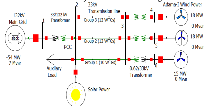
Fig.3.7. System model for steady state voltage
