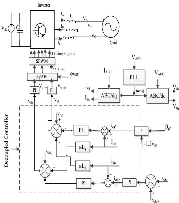
Fig.2.5. Voltage-oriented with a decoupled controller
