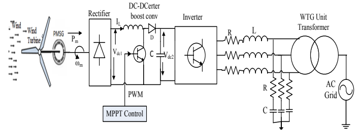
Fig.1.2. Single line electrical diagram of 1.5MW Adama-I WTG
