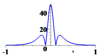
Fig.1. The plot of graph of the absolute value of the second derivative of the Runge function.
