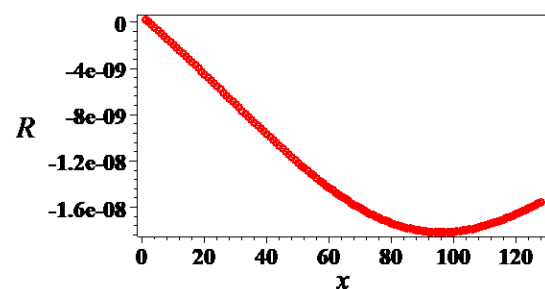
Fig.13. The plot of error between the exact solution of the equation (problem 1) and the numerical solution obtained with the application of the polynomial splines of the third order approximation when we use 128 nodes.
