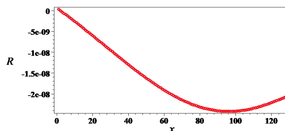
Fig.10. The plot of error between the exact solution of the equation (problem 1) and the numerical solution obtained with the application of the non-polynomial splines ( \varphi_1(x) = 1 , \varphi_2(x) = \sin(x) , \varphi_3(x) = \cos(x) ) when we use 128 nodes
