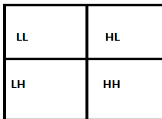
Figure 17: Sub-bands 2D-DWT
